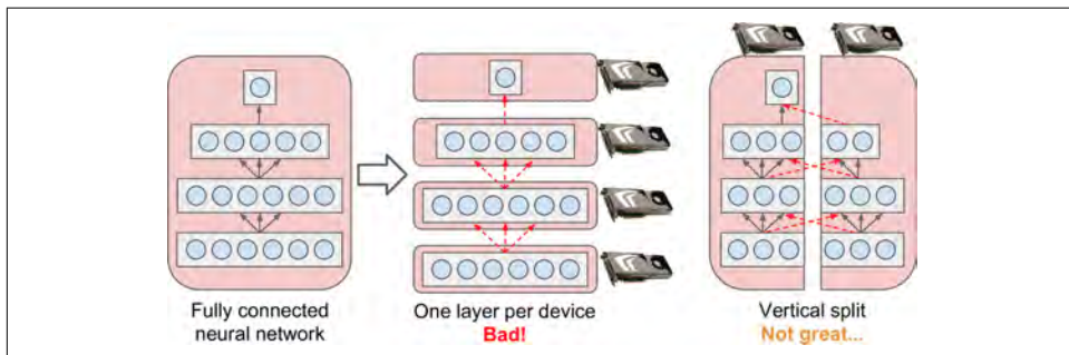
Figure 12-14. Splitting a fully connected neural network
