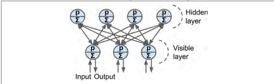
Figure E-3. Restricted Boltzmann machine
